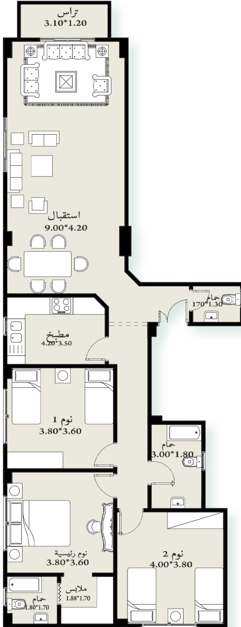
TYPICAL FLOOR
